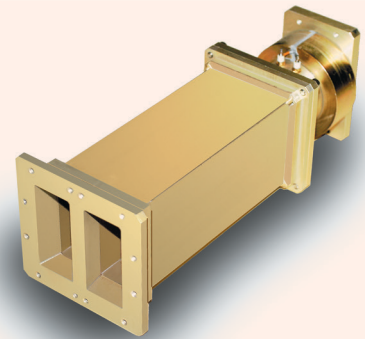
C-Band Constant Current SPDT Switch
