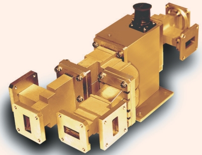
X-Band Constant Current DP4T Switch
