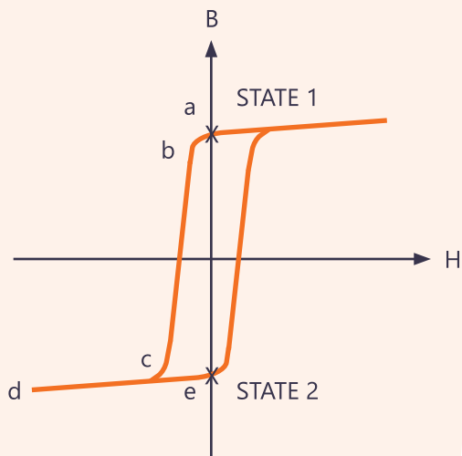
Figure 3 - Hysteresis Loop
