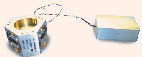
X-Band Switching Circulator
